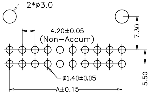
RECOMMENDED P. C. B HOLE PATTERN
